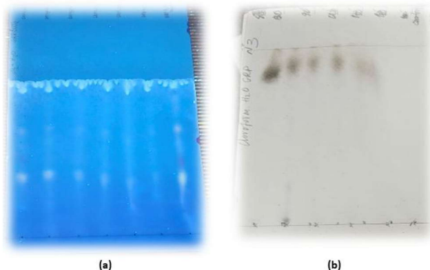
Figure 1 – TLC of extracts obtained by SCFE using CO 2 +H 2 O binary co-solvent system: (a) in S 2 -based system; and (b) chloroform-based system.
