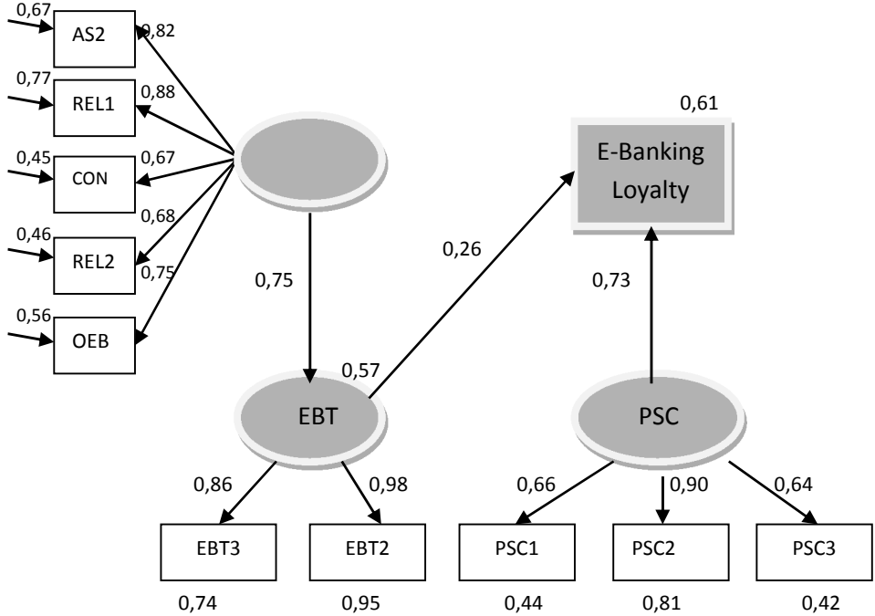
Figure 5- Online Structural Equation -Model B
