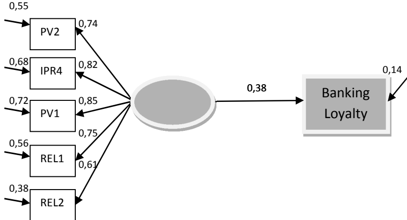
Figure 4- Offline Structural Equation- Model A
