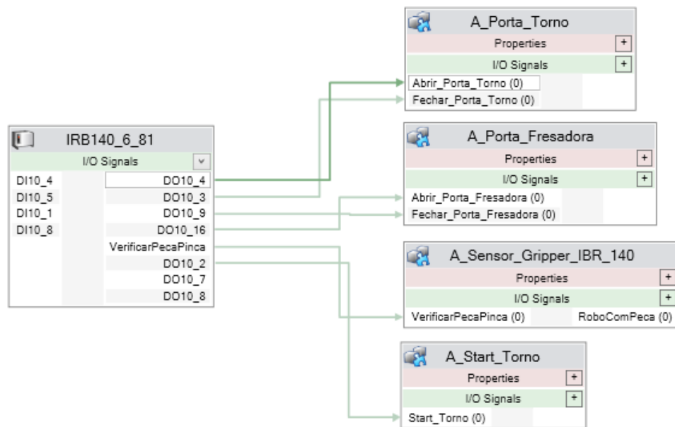
Figura 58: Station Logic no RobotStudio.
