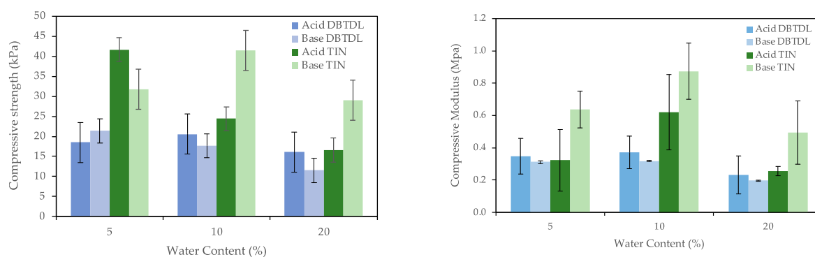
Figure 1. Compressive strength and compressive modulus of PUF made with different amounts of blowing agent (water). It was prepared using as a base 4 g of polyol, 11 g of isocyanate, 0.2 g of catalyst (TIN and DBTDL), 0.28 g of surfactant, and the blowing agent varied from 0.2 to 0.8 g.
