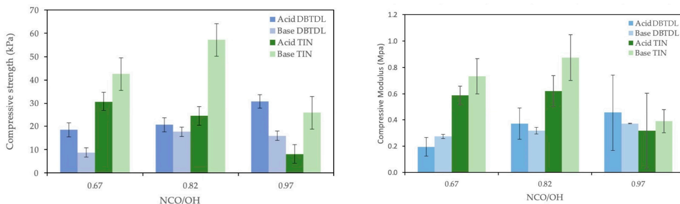
Figure 2. Compressive strength and compressive modulus of PUF made with different isocyanate indices. It was prepared using 4 g of polyol, 0.4 g of various blowing agents, 0.2 g of catalyst (TIN and DBTDL), 0.28 g of surfactant, and isocyanate ranging from 9 to 13 g.
