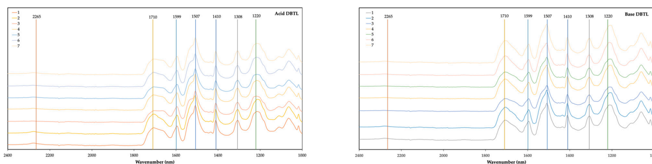
Figure 4. FTIR spectra of foams using acid-liquefied polyol (left) and base-liquefied polyol (right) and DBTDL as catalyzer. (1) Base foam with 10% water, surfactant (7%), catalyzer (5%), and NCO index 0.8; (2) water 5%; (3) water 15%; (4) 2.5% catalyzer; (5) 10% catalyzer; (6) NCO index 0.7; (7) NCO index 1.
