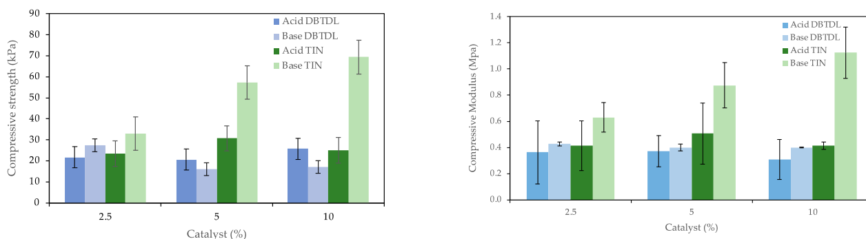
Figure 3. Compressive strength and compressive modulus of PUF made with different amounts of catalyst (DBTDL) for TIN catalyst. It was prepared using as a base 4 g of polyol, 0.4 g of various blowing agents, 0.28 g of surfactant, 11 g of isocyanate, and the catalyst varied from 0.1 to 0.8 g for TIN and DBTDL.
