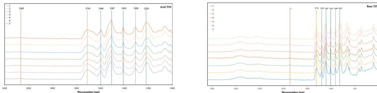
Figure 5. FTIR spectra of foams using acid-liquefied polyol ( left ) and base-liquefied polyol ( right ) and TIN as catalyst. (1) Base foam with 10% water, surfactant (7%), catalyst (5%) and NCO index 0.8; (2) water 5%; (3) water 15%; (4) 2.5% catalyst; (5) 10% catalyst; (6) NCO index 0.7; (7) NCO index 1.
